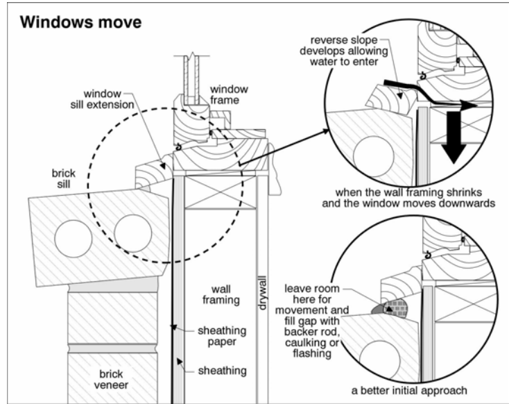
Drawing - Window movement
